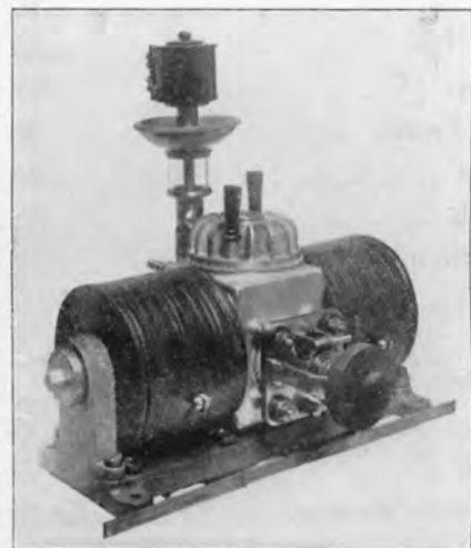
2 Kw. ARC CONVERTER
