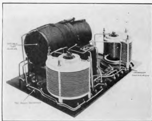
INTERNAL VIEW SIMON U. S. ARMY RECEIVER
