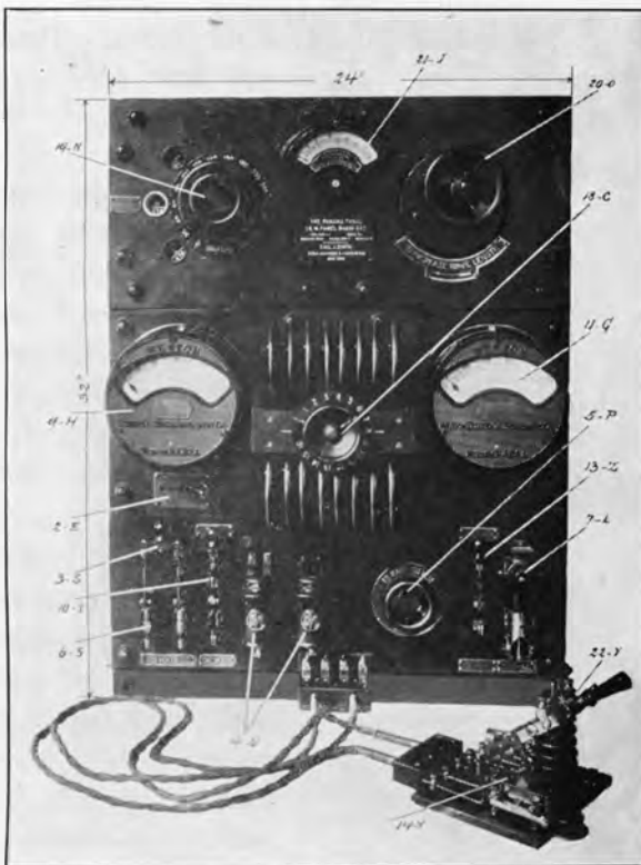
SIMON PANAMA CANAL 1 Kw. TRANSMITTER
