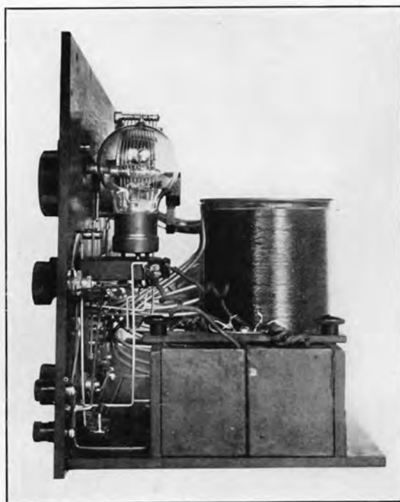
RIGHT SIDE INTERNAL VIEW FRENCH MARINE RECEIVER
