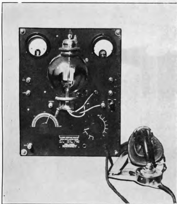
ORIGINAL AIRCRAFT RADIO TELEPHONE TRANSMITTER
