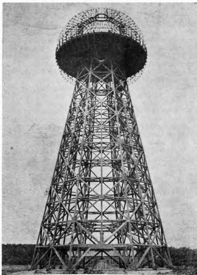
TESLA CENTRAL POWER PLANT AND TRANSMITTING TOWER FOR WORLD TELEGRAPHY LONG ISLAND, N. Y.
